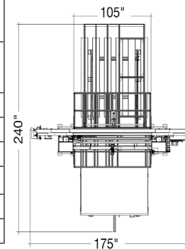
Footprint / Vista Superior 11385-X & X-O
