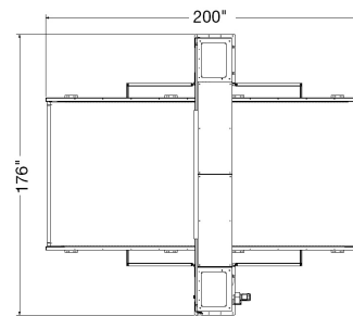
Footprint / Vista Superior
