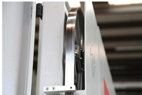
Circulating bandknife Cuchilla circular
