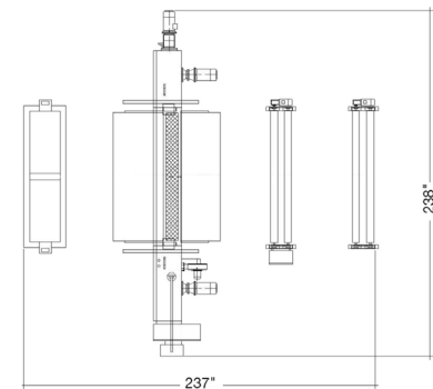
Footprint with winder/unwinder Vista Superior con enrollado/desenrollado
