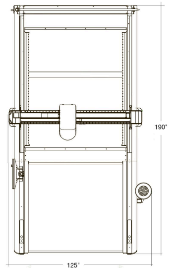
Foot print / Vista Superior
