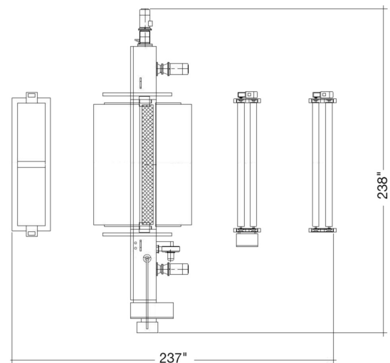
Footprint with winder/ unwinder Visa Superior con enrollado/desenrollado
